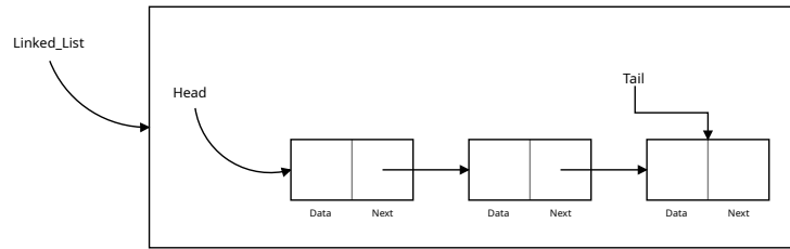
Figure 94: Double-Ended Linked List Reference Image
